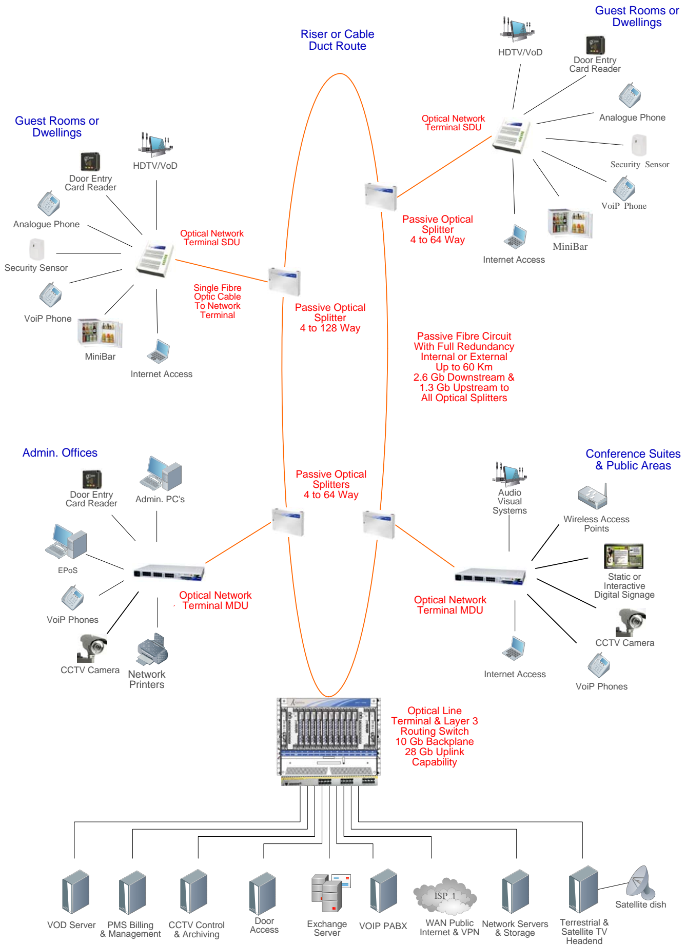
G-PON Unified Communication Network Hotel / Resort or Campus Application
